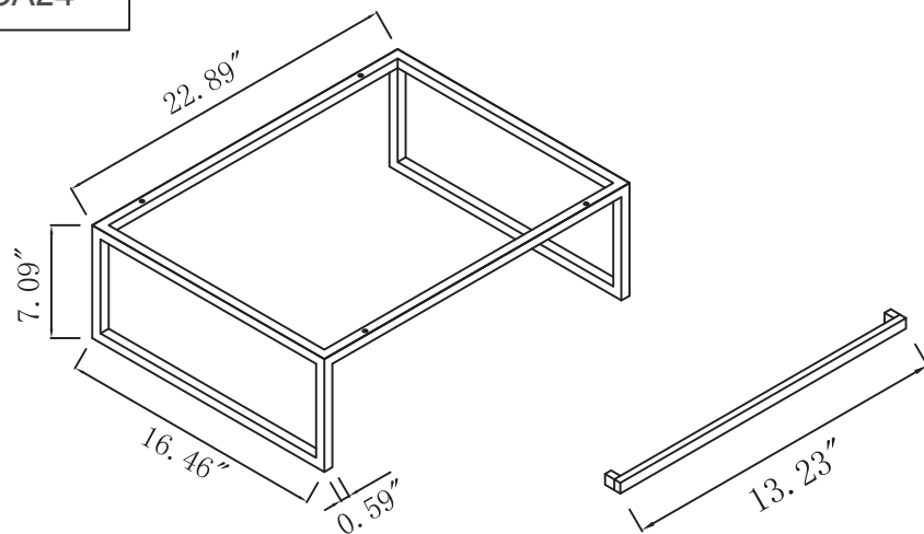
Stainless steel frame
