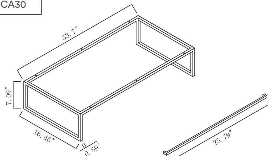
Stainless steel frame
